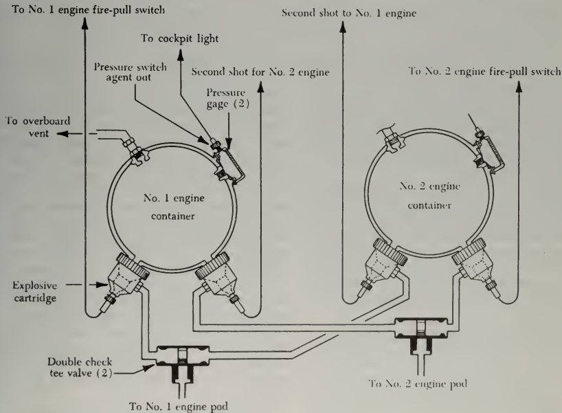
FIGURE 9-12. Fire extinguisher system for a multi-engine aircraft.
